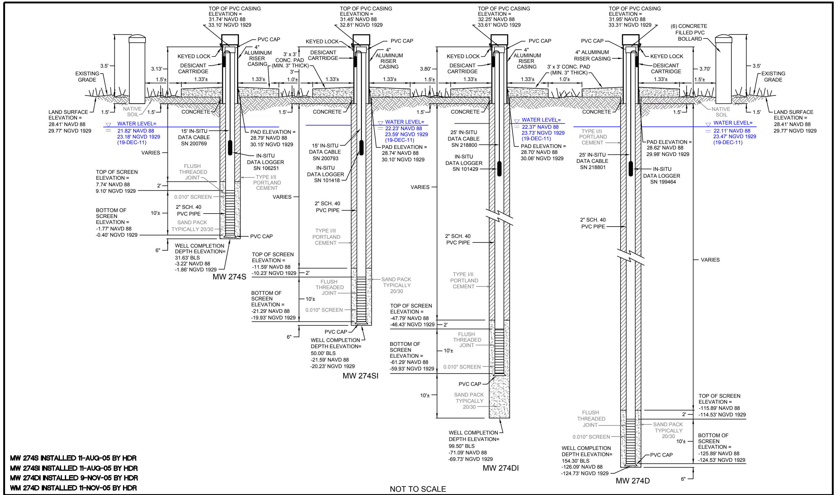
Figure 3-6 Well Construction Detail Old Well ID: MW 274S, MW 274SI, MW 274DI & MW 274D DBHYDRO ID: C44B2A1, C44B2A2, C44B2A3 & C44B2A4
