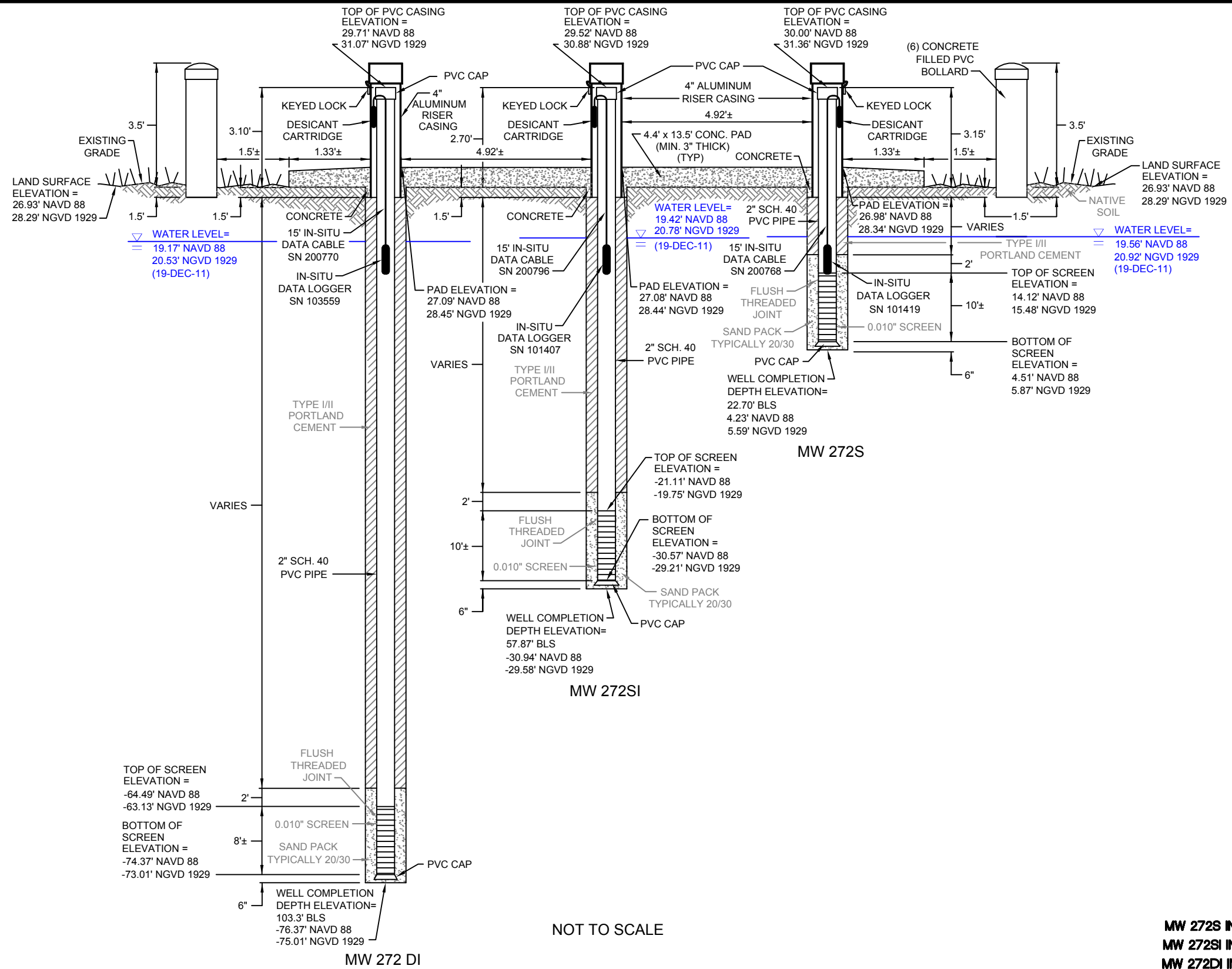
Figure 3-8 Well Construction Detail Old Well ID: MW 272S, MW 272SI & MW 272DI DBHYDRO ID: C44B8D1, C44B8D2 & C44B8D3
