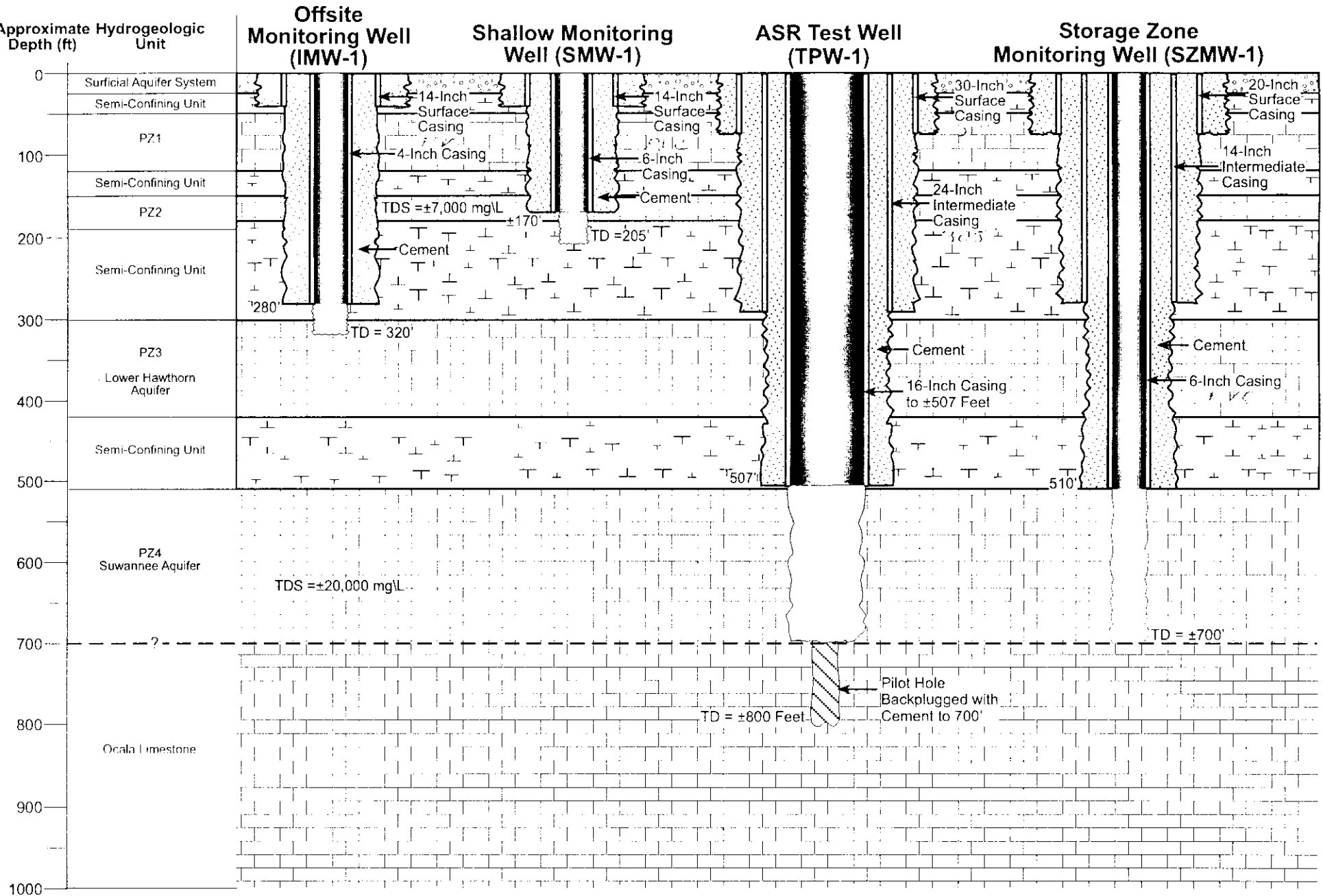
FIGURE 5-1 ASR System Well Construction Details
