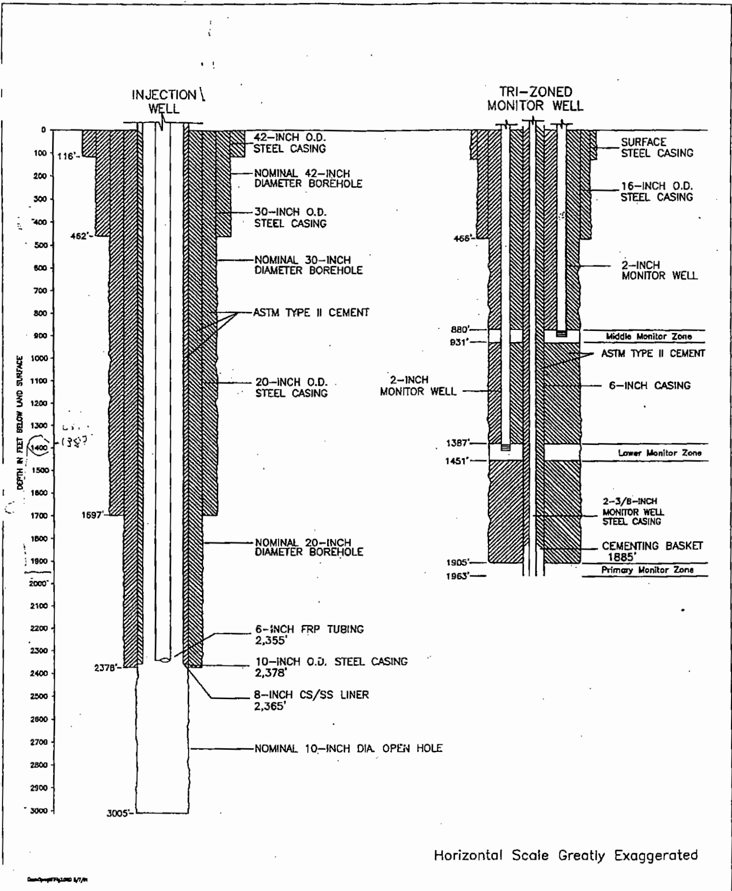
FIGURE 8 WELL CONSTRUCTION DIAGRAMS INJECTION AND MONITOR WELLS OCEAN SPRAY CRANBERRIES, INC VERO BEACH, FLORIDA
