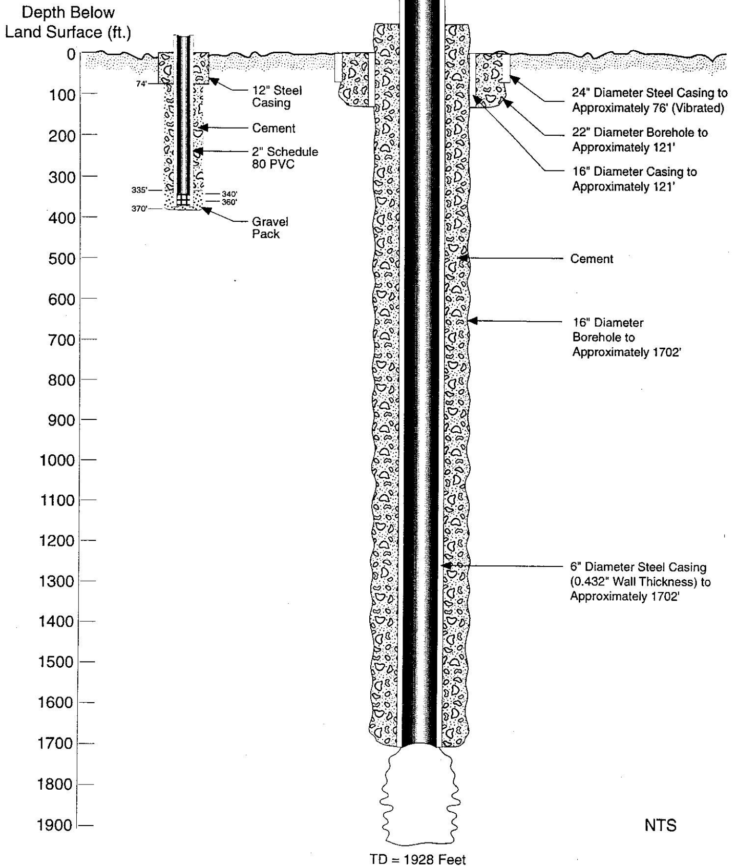
FIGURE 2-2 Class I Injection Well and Monitoring Well Construction Details at the GIWA WWTP
