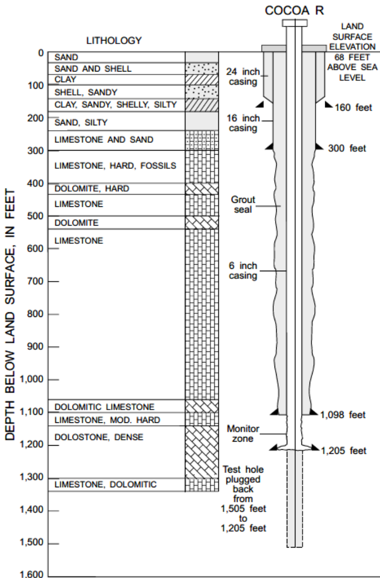
Figure 22. Geohydrologic section showing well-completion data for well R
