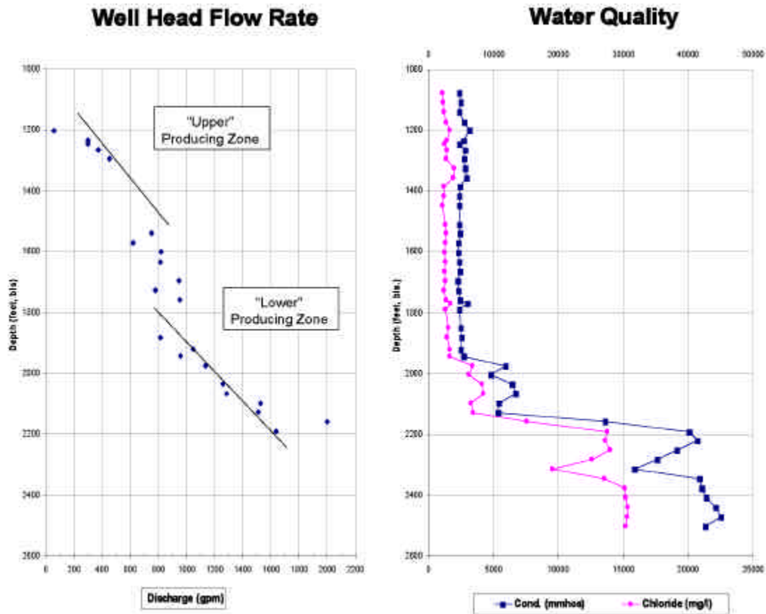
Figure 7. Wellhead Water Quality and Flow Rate as a Function of Depth
