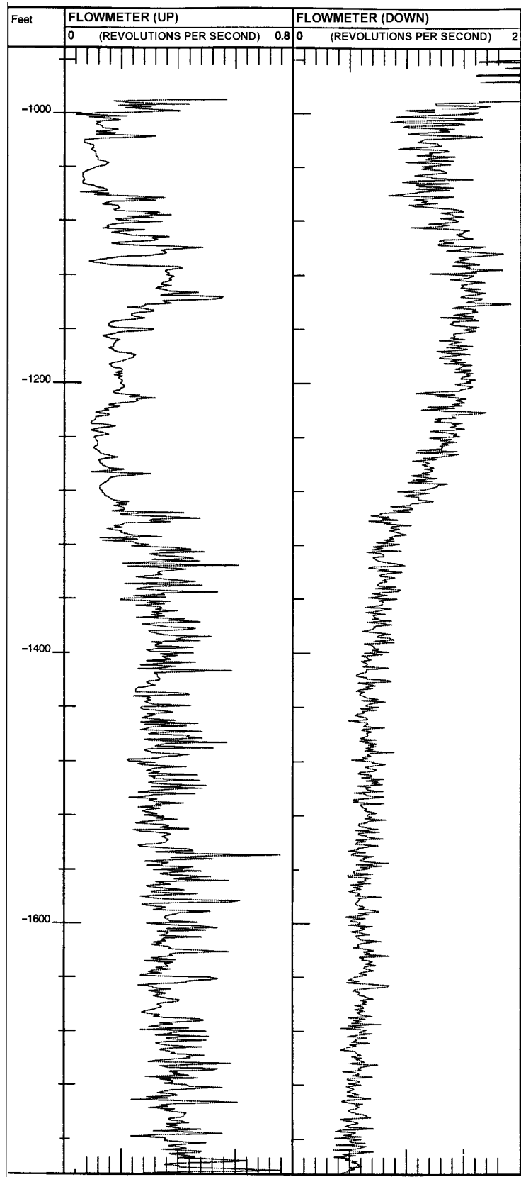
Figure B-4. Geophysical Log of PBF-7 (Sheet 4 of 5)
