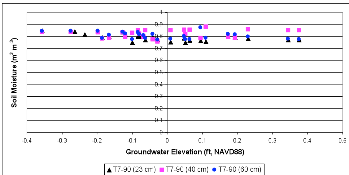
Figure 33. Mean monthly groundwater elevation at well T7-W03 (ft, NAVD88) versus mean monthly soil moisture ( \text{m}^3 \text{m}^{-3} ) measured at station T7-90.
