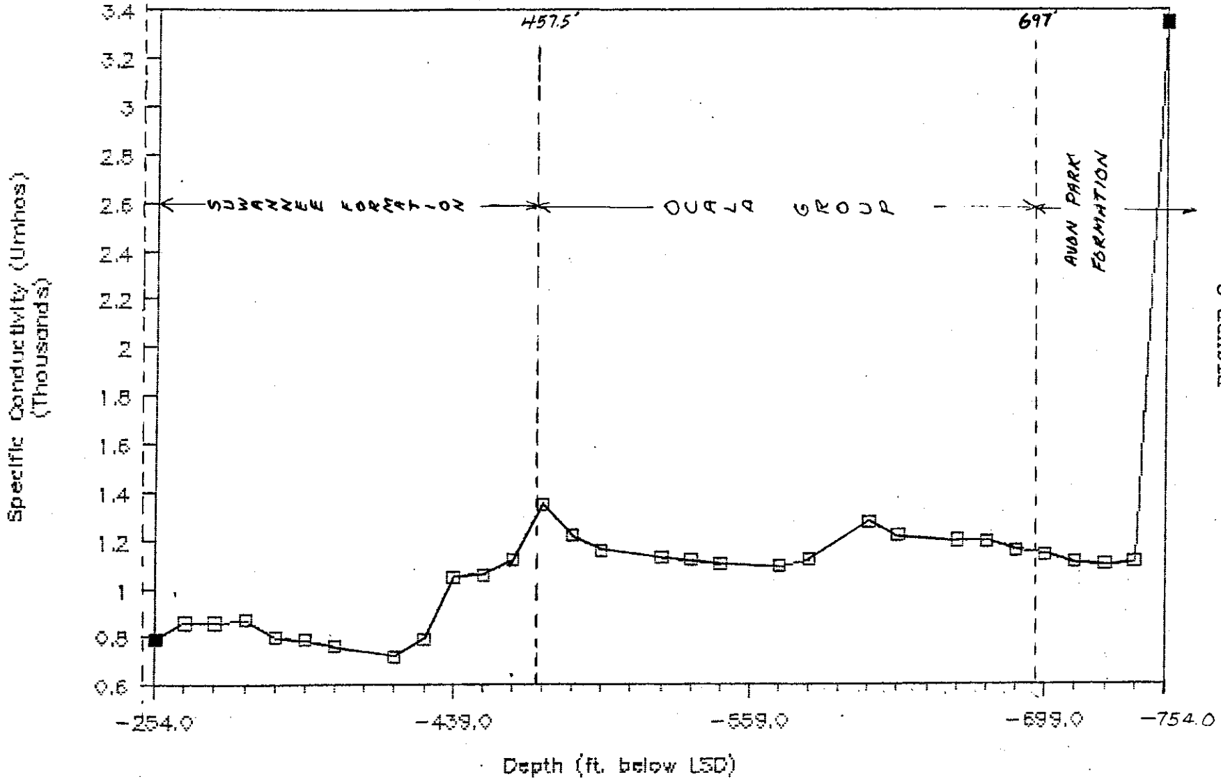
Specific Conductivity vs Depth
