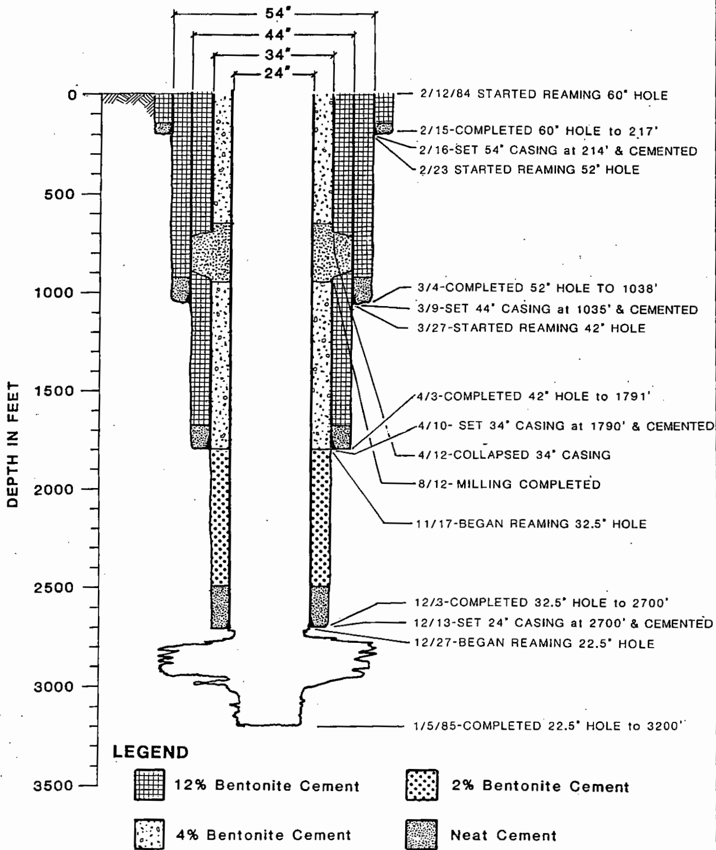
WELL COMPLETION DIAGRAM FOR IW-1
