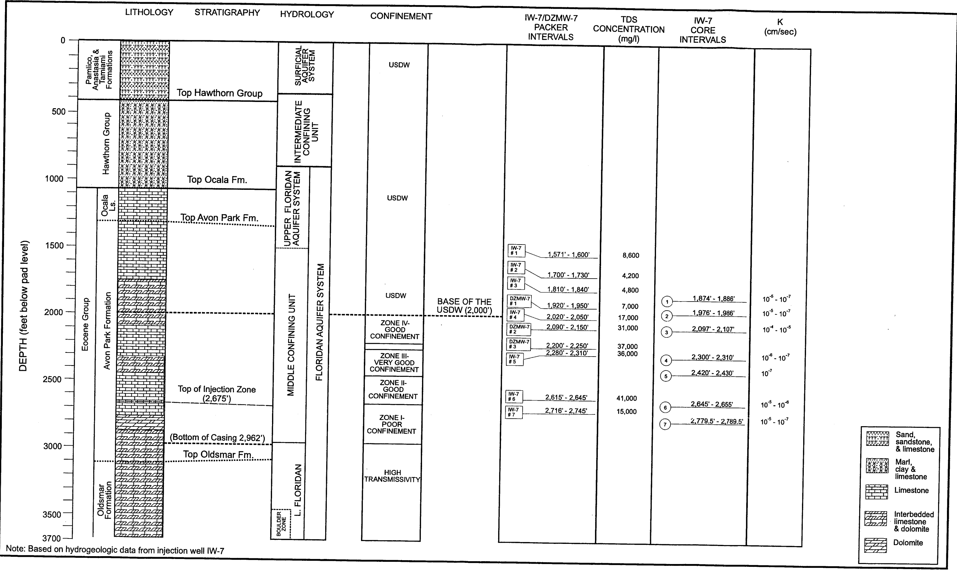
Figure No. 2-1 City of WPB ECRWWTP, Florida Geologic Column for IW-7
