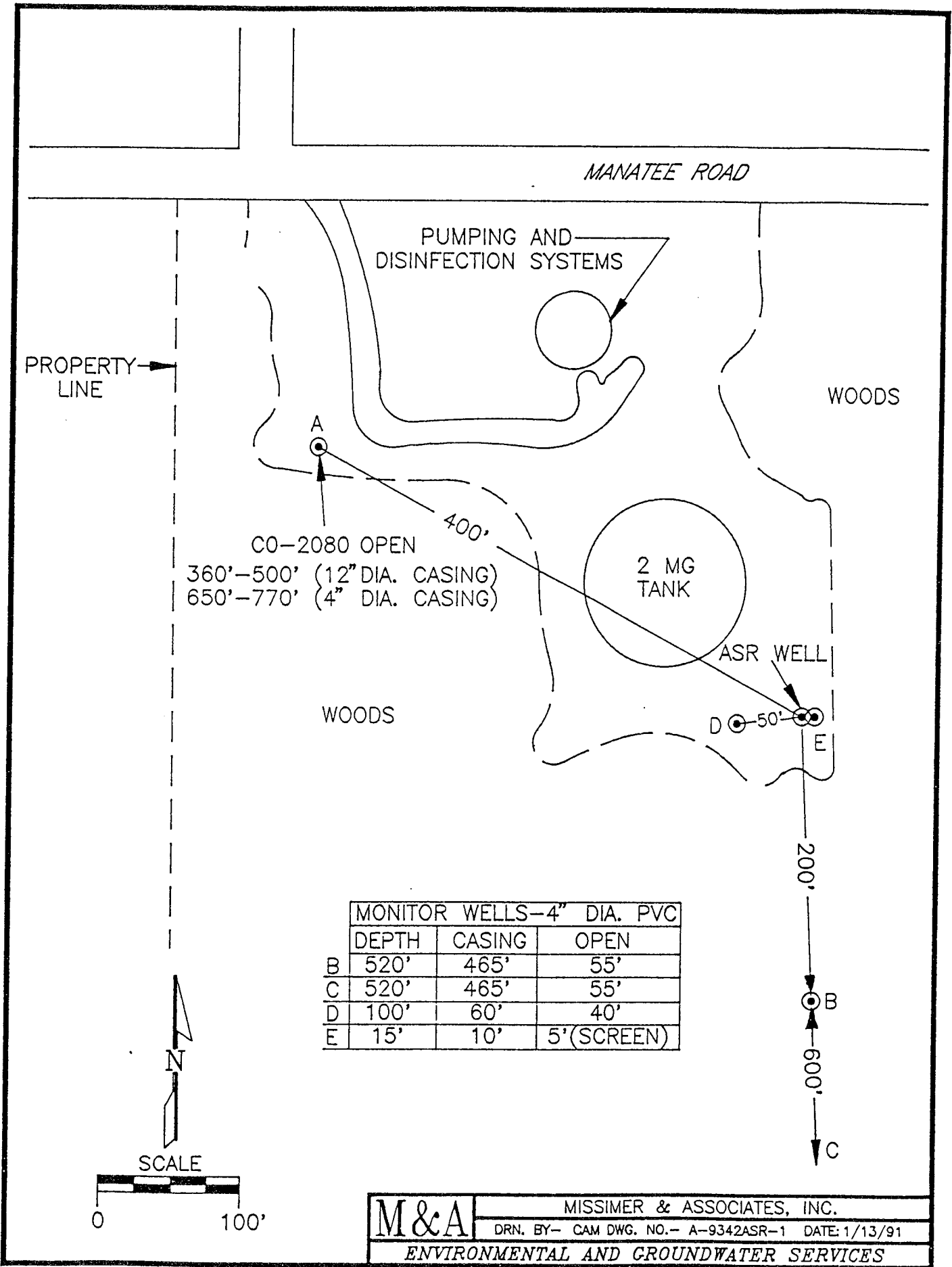
FIGURE A-1. PROPOSED ASR WELL AND MONITORING WELL LOCATIONS.
