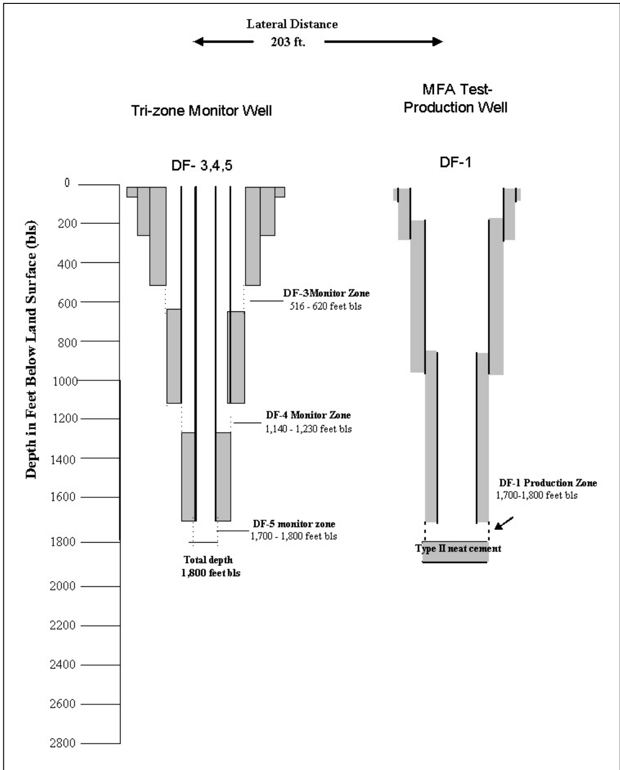
Figure 21. Well Configuration- APT-2.
