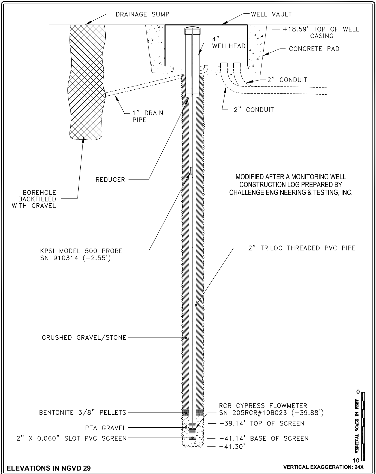
FIGURE 5-2. MONITORING WELL MW-2 CONSTRUCTION DETAILS.
