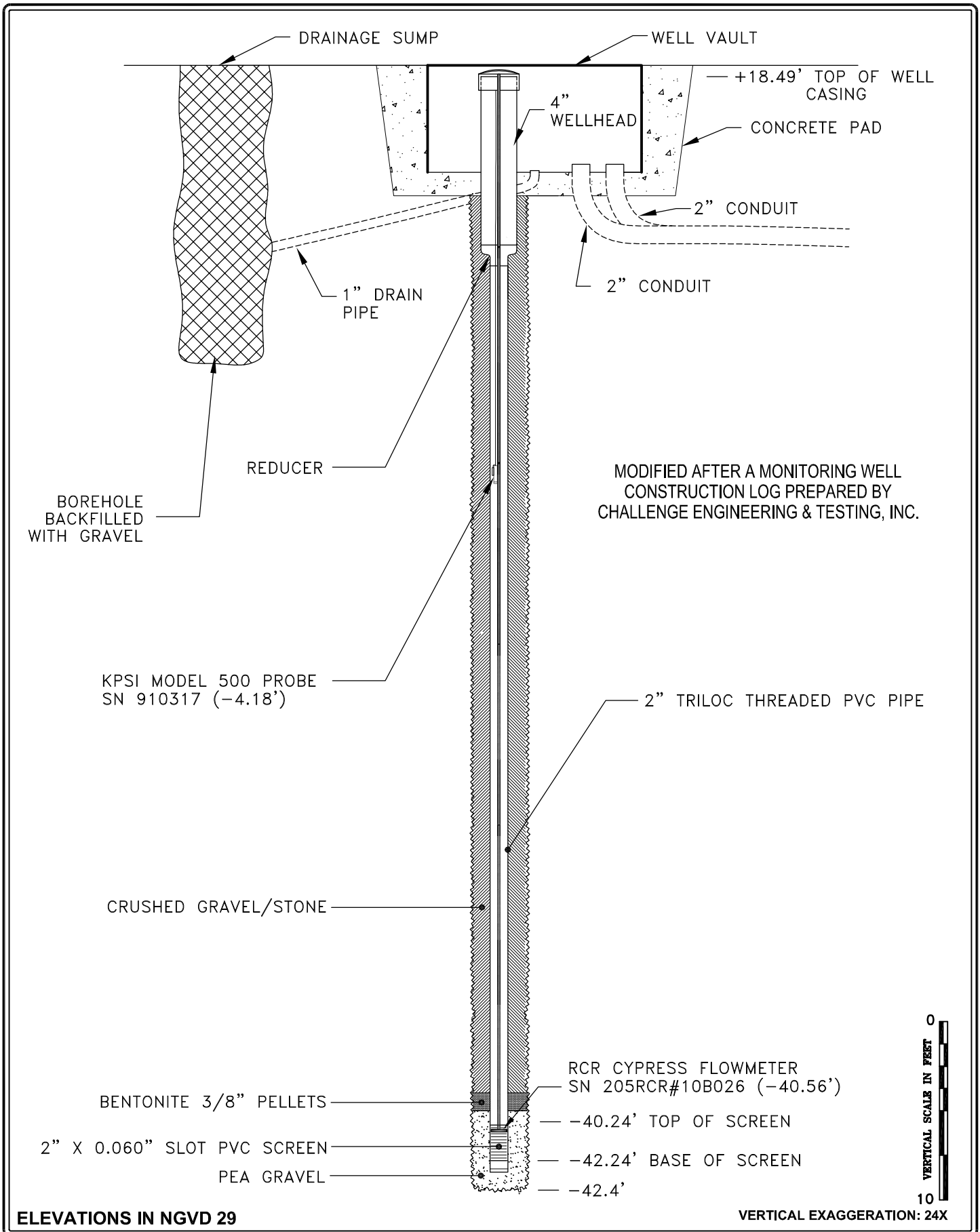
FIGURE 5-3. MONITORING WELL MW-3 CONSTRUCTION DETAILS.
