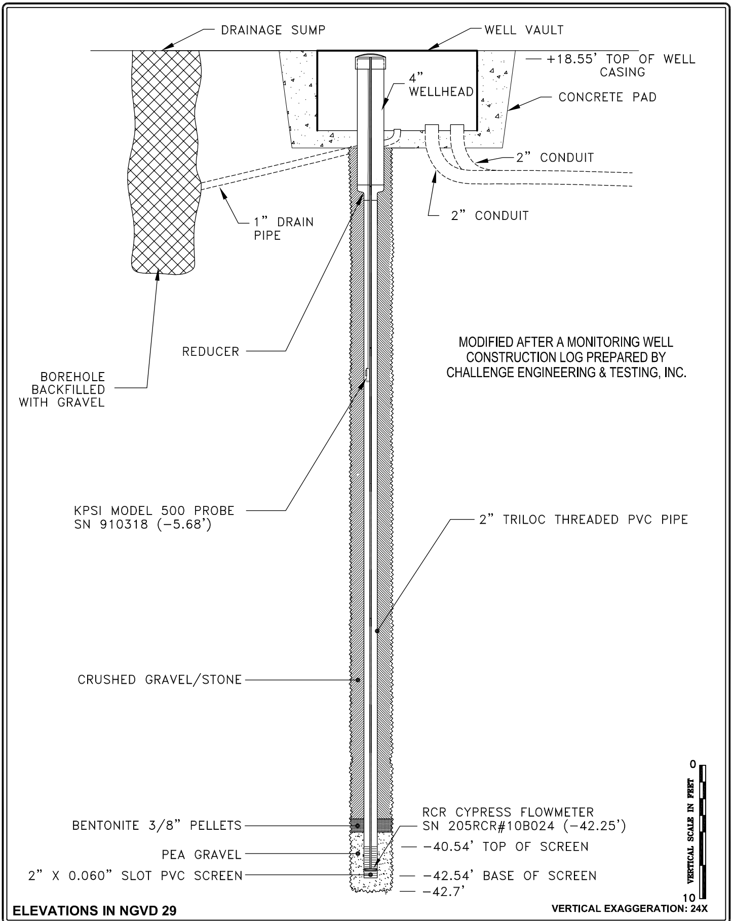
FIGURE 5-1. MONITORING WELL MW-1 CONSTRUCTION DETAILS.
