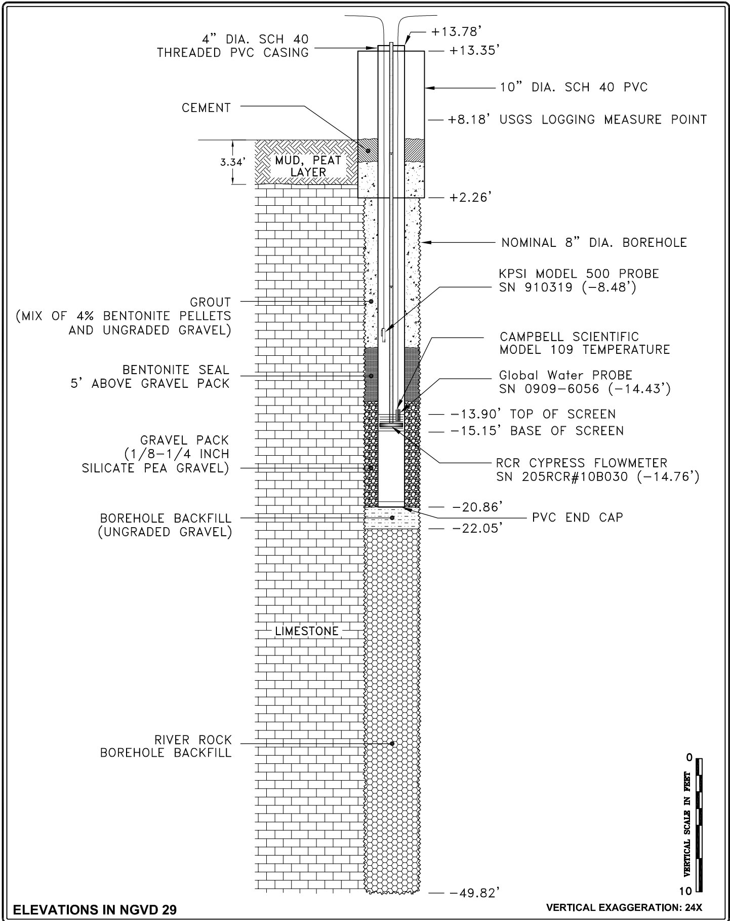
FIGURE 5-8. MONITORING WELL MW-8 CONSTRUCTION DETAILS.
