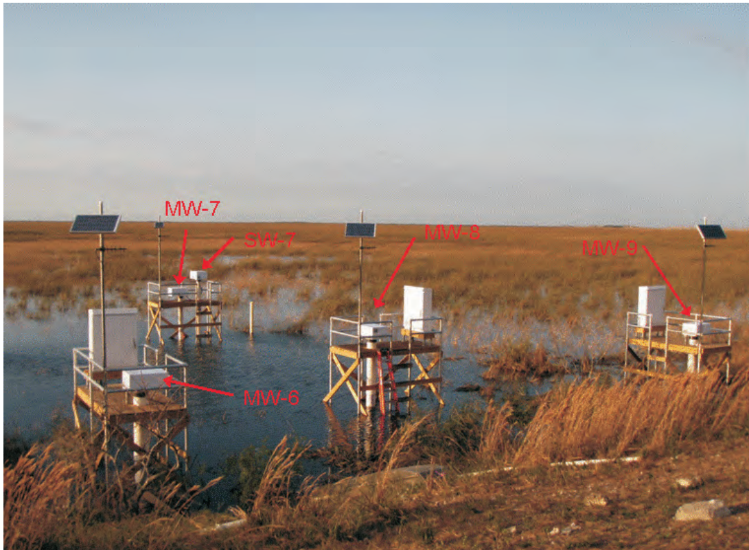
L-30 Seepage Management Pilot Project – Monitoring Wells Installed In the Planned Cutoff Wall Window Nov 2009-Feb 2010 for Baseline Monitoring
