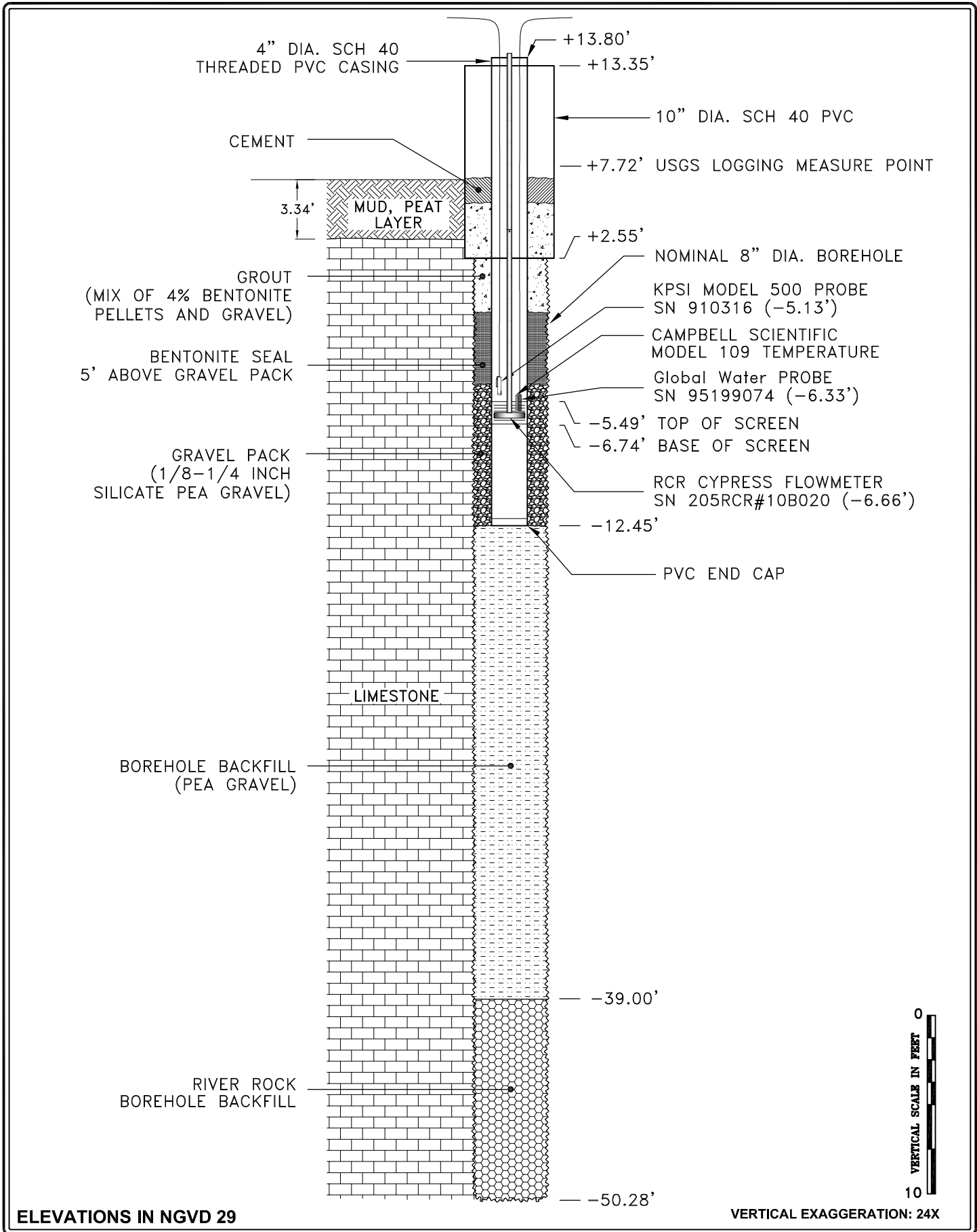
FIGURE 5-9. MONITORING WELL MW-9 CONSTRUCTION DETAILS.
