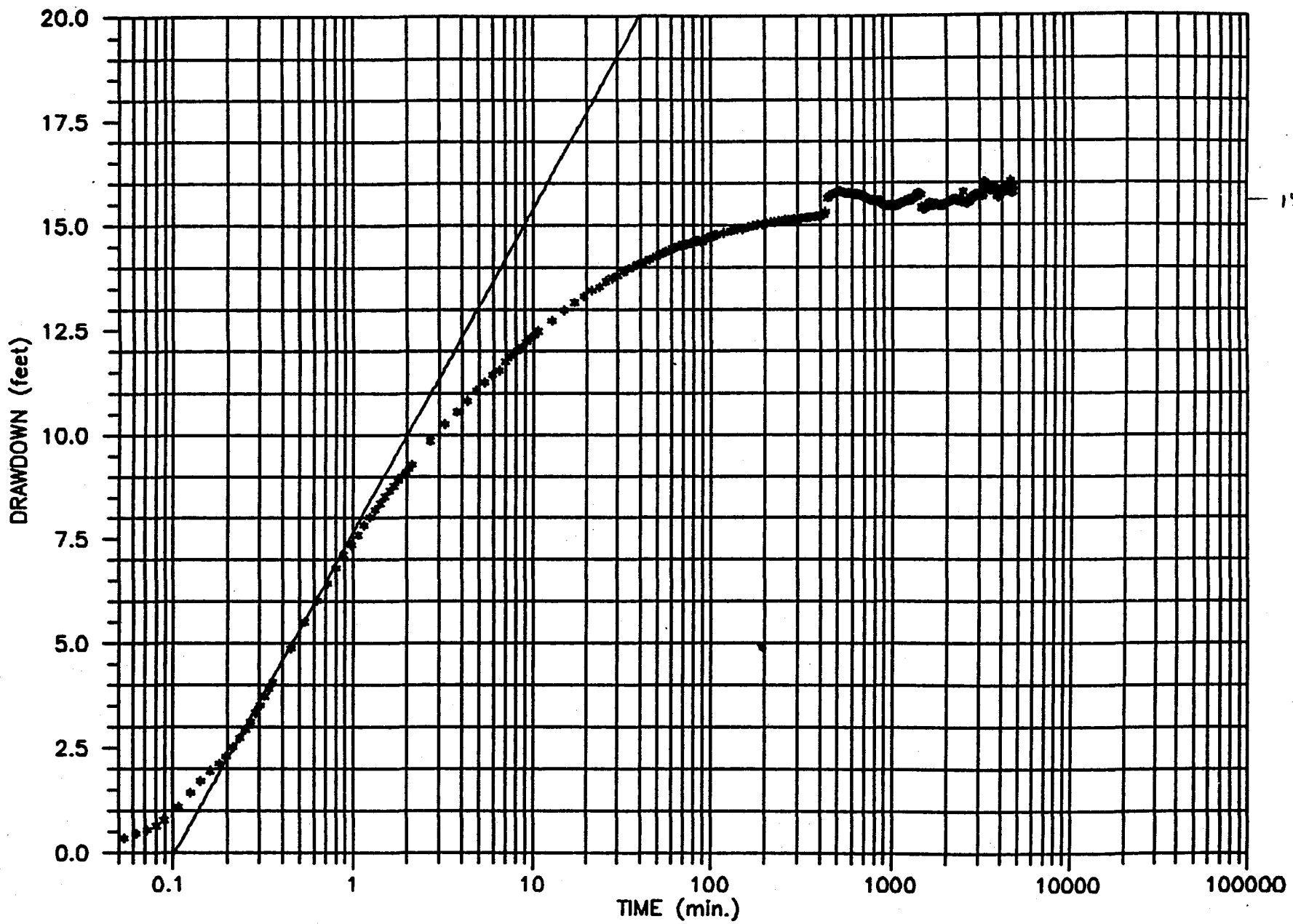
TIME - DRAWDOWN SEMI-LOG PLOT FOR WELL PZ36D
