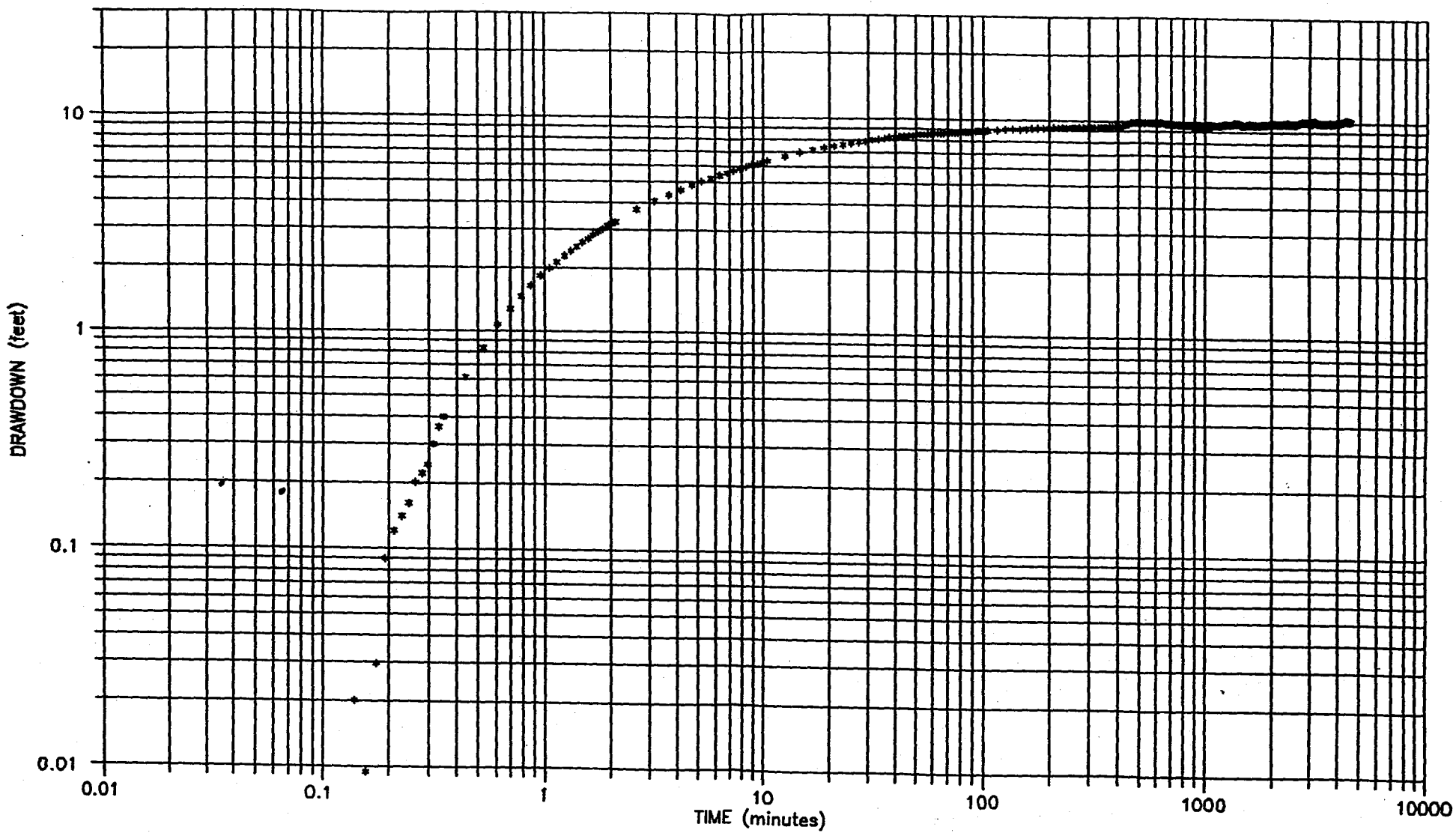
WELL PZ87D TIME - DRAWDOWN PLOT FIGURE 5-14
