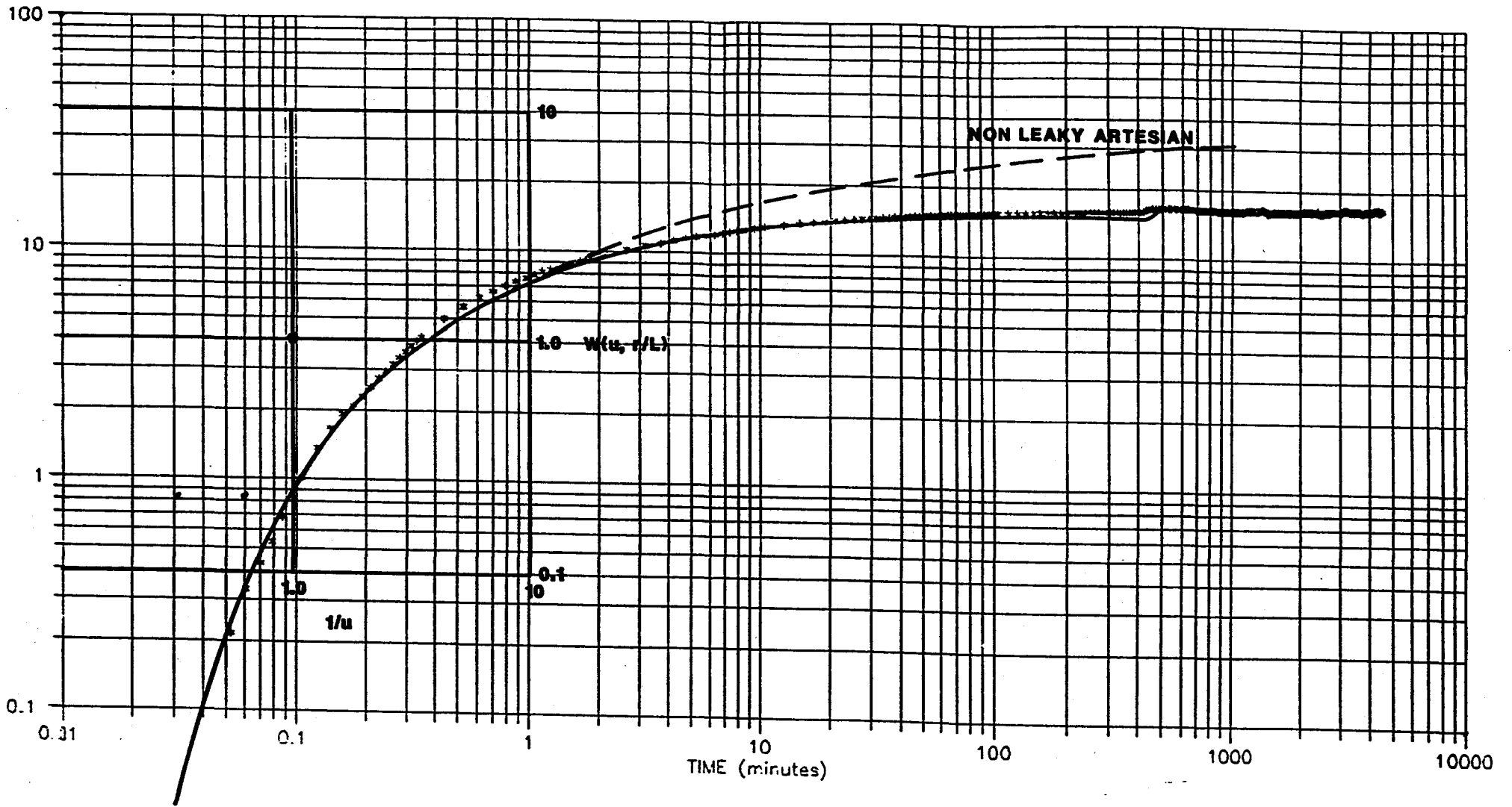
LOG-LOG PLOT OF DRAWDOWN VS. TIME FOR WELL PZ36D WITH A COMPARISON TO WALTON LEAKY CURVE, r/L = 0.2 ( Q = 395 GPM)
