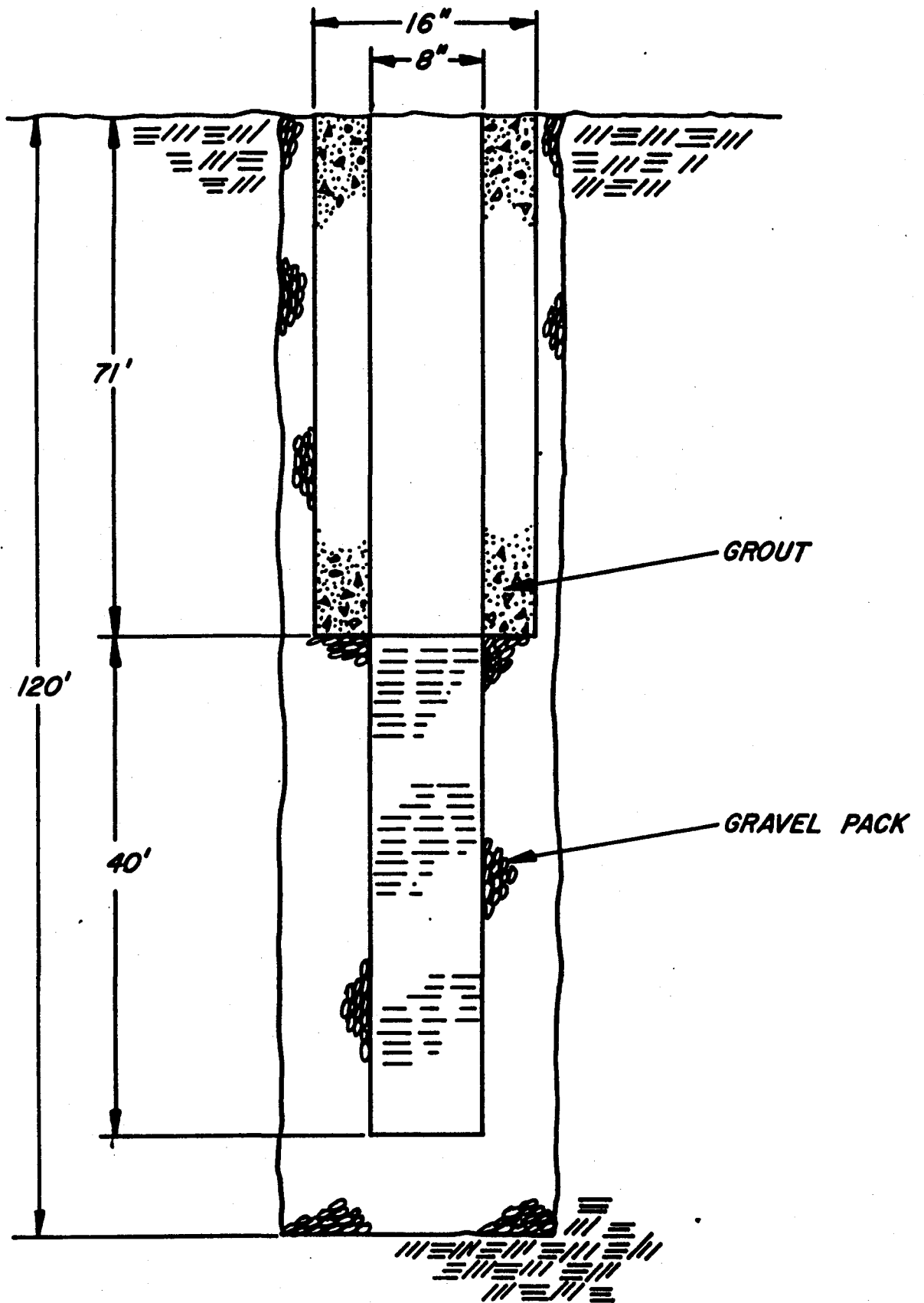
PRODUCTION WELL 7 CONSTRUCTION DIAGRAM
