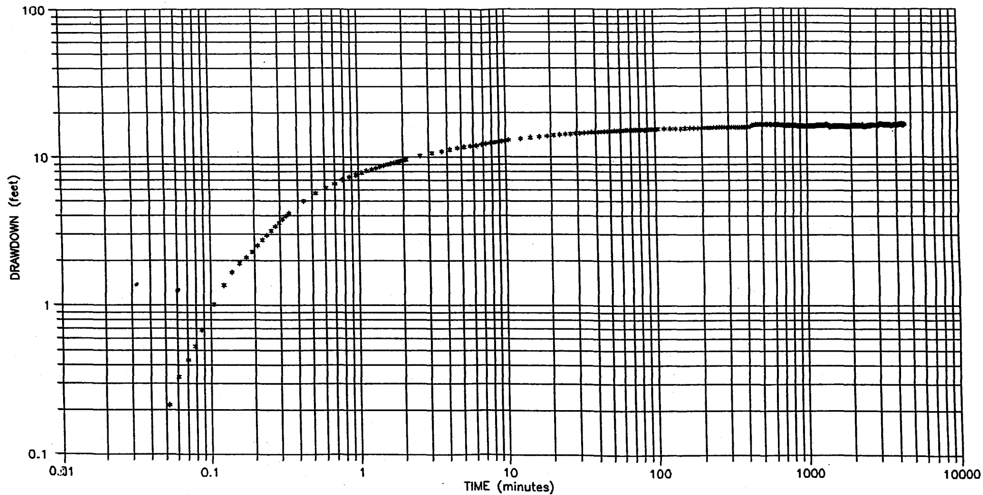
WELL PZ36D TIME - DRAWDOWN PLOT FIGURE 5-12
