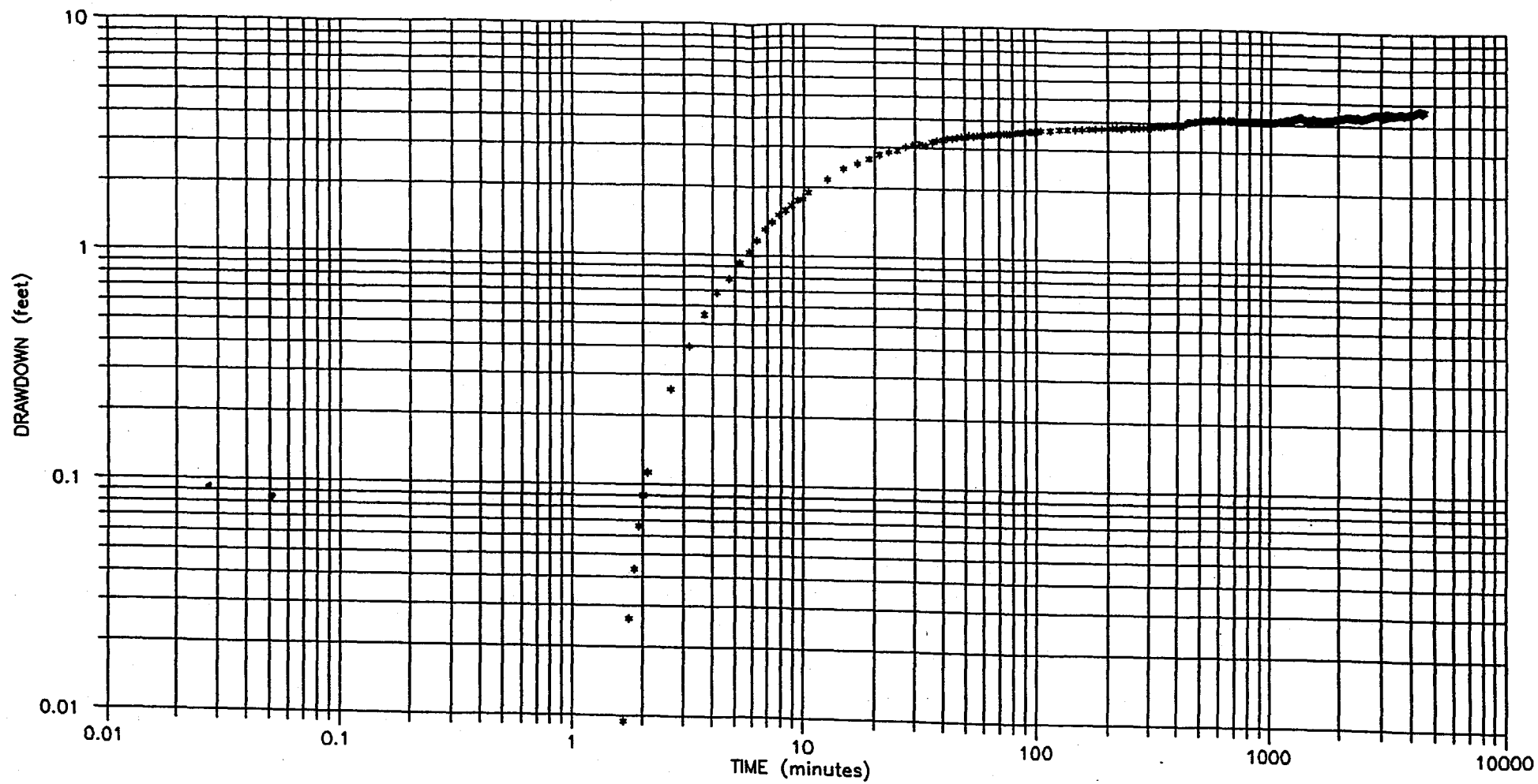
WELL PZ871 TIME - DRAWDOWN PLOT FIGURE 5-15
