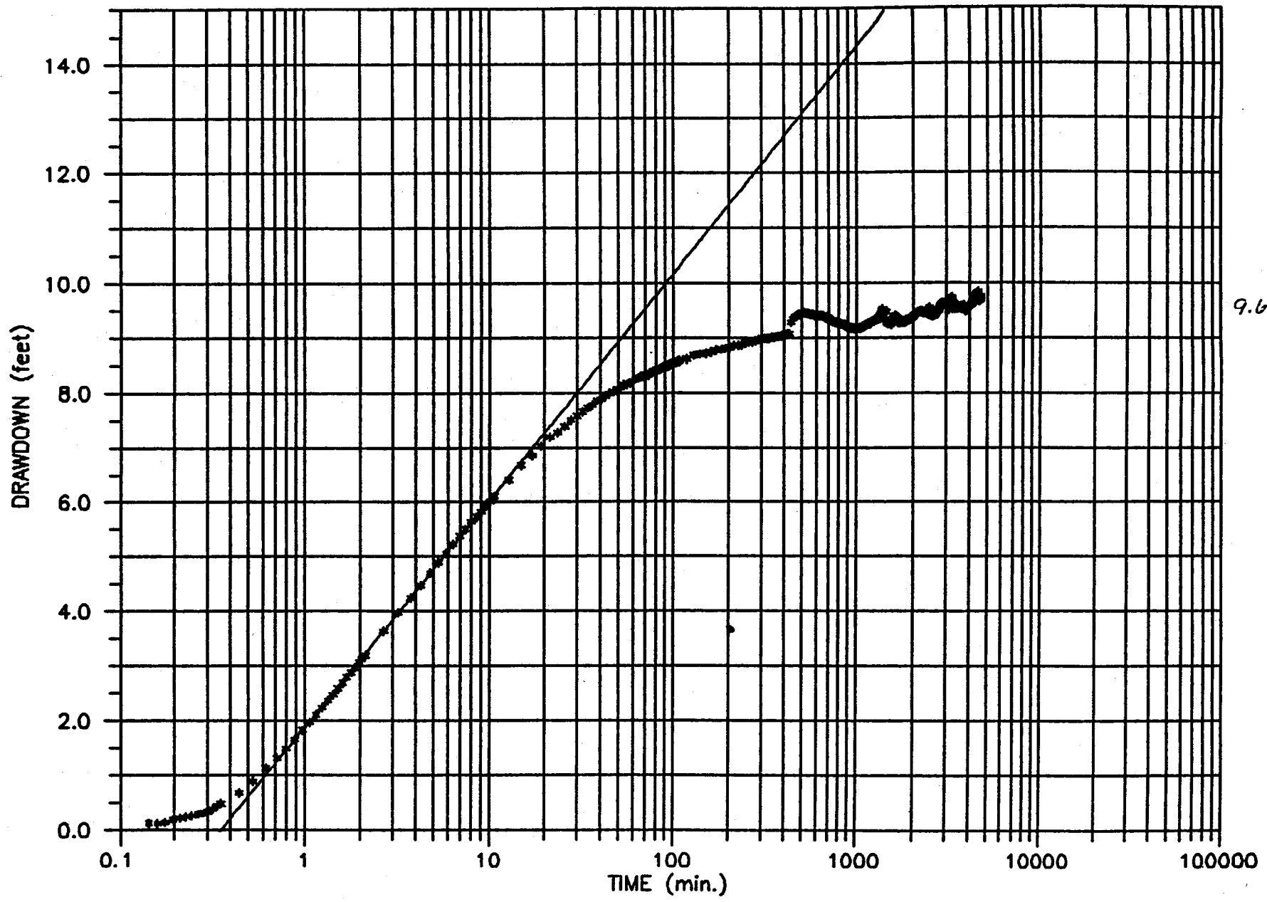
TIME - DRAWDOWN SEMI-LOG PLOT FOR WELL PZ87D
