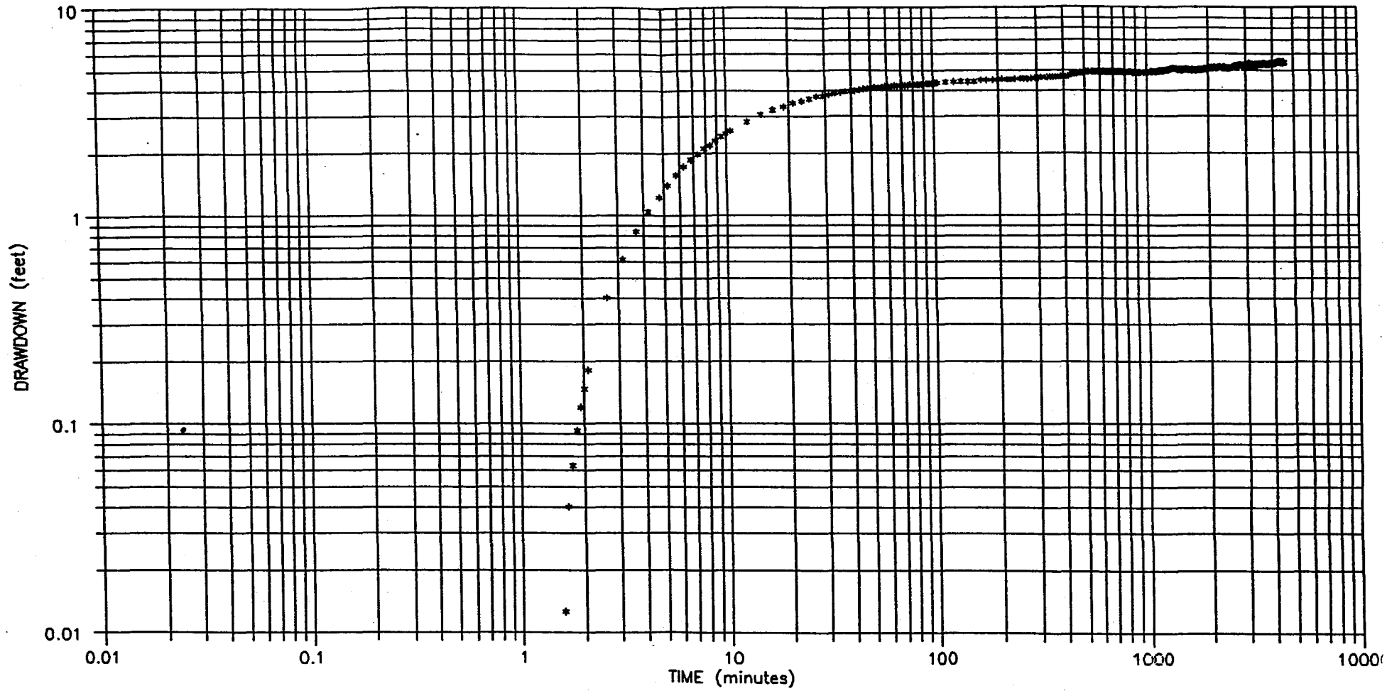
WELL PZ36I TIME - DRAWDOWN PLOT FIGURE 5-13
