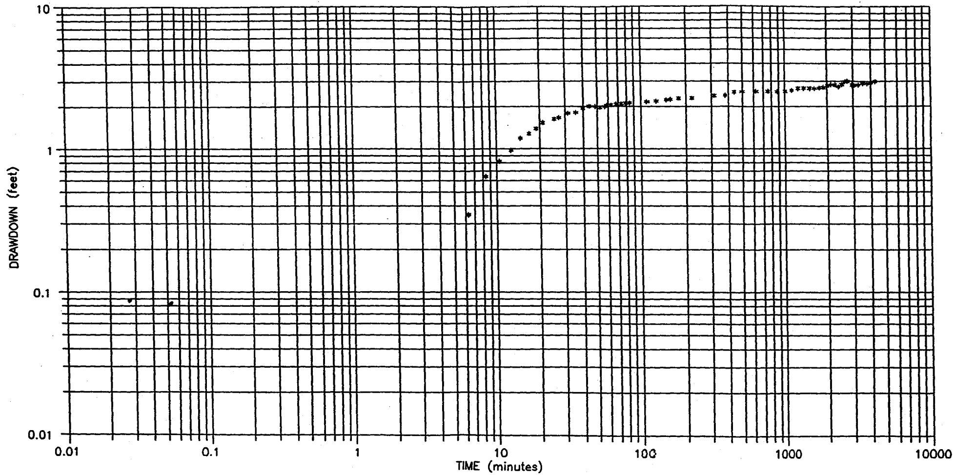
WELL PZ136I TIME - DRAWDOWN PLOT FIGURE 5-17
