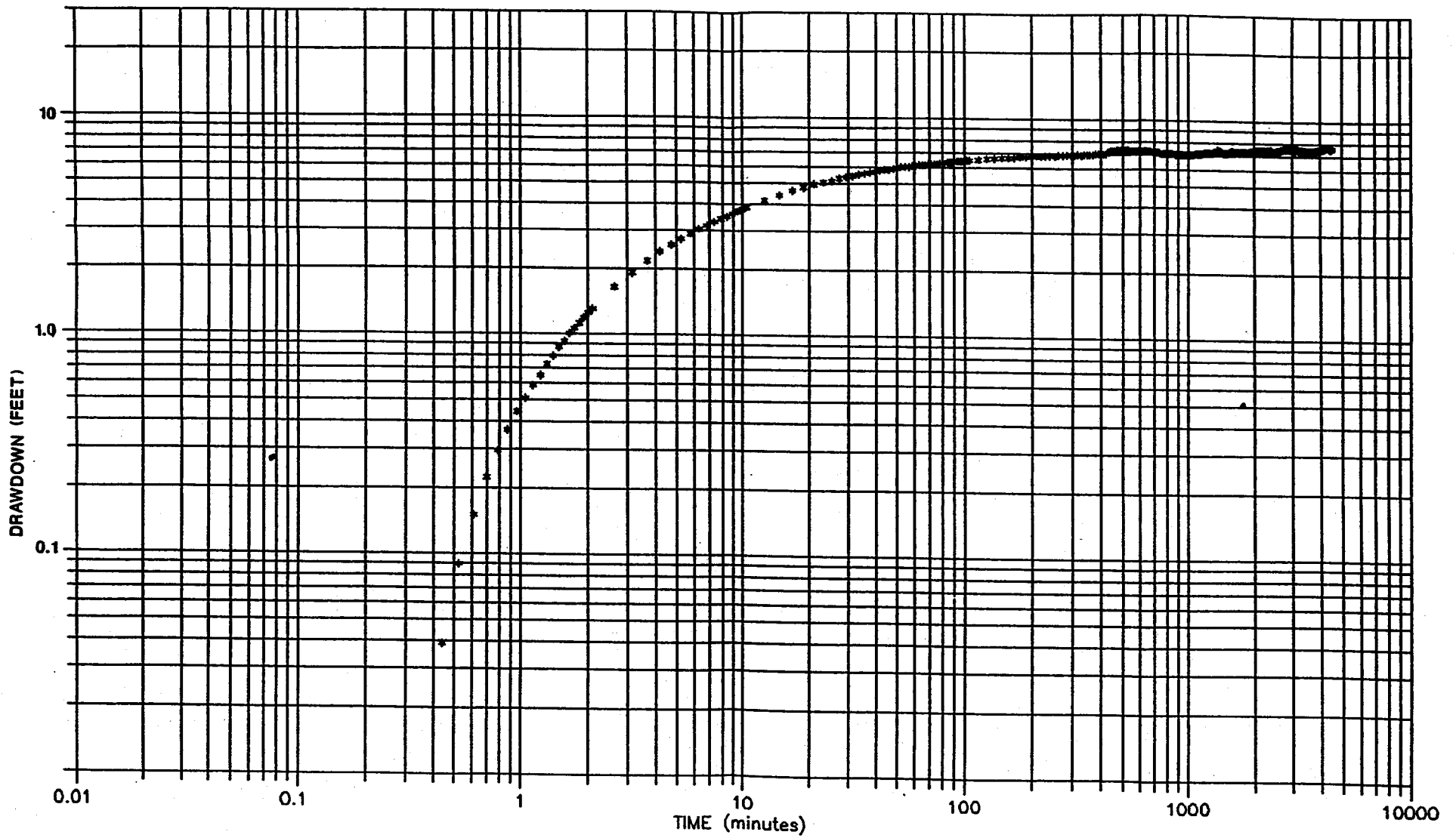
WELL PZ136D TIME - DRAWDOWN PLOT FIGURE 5-16
