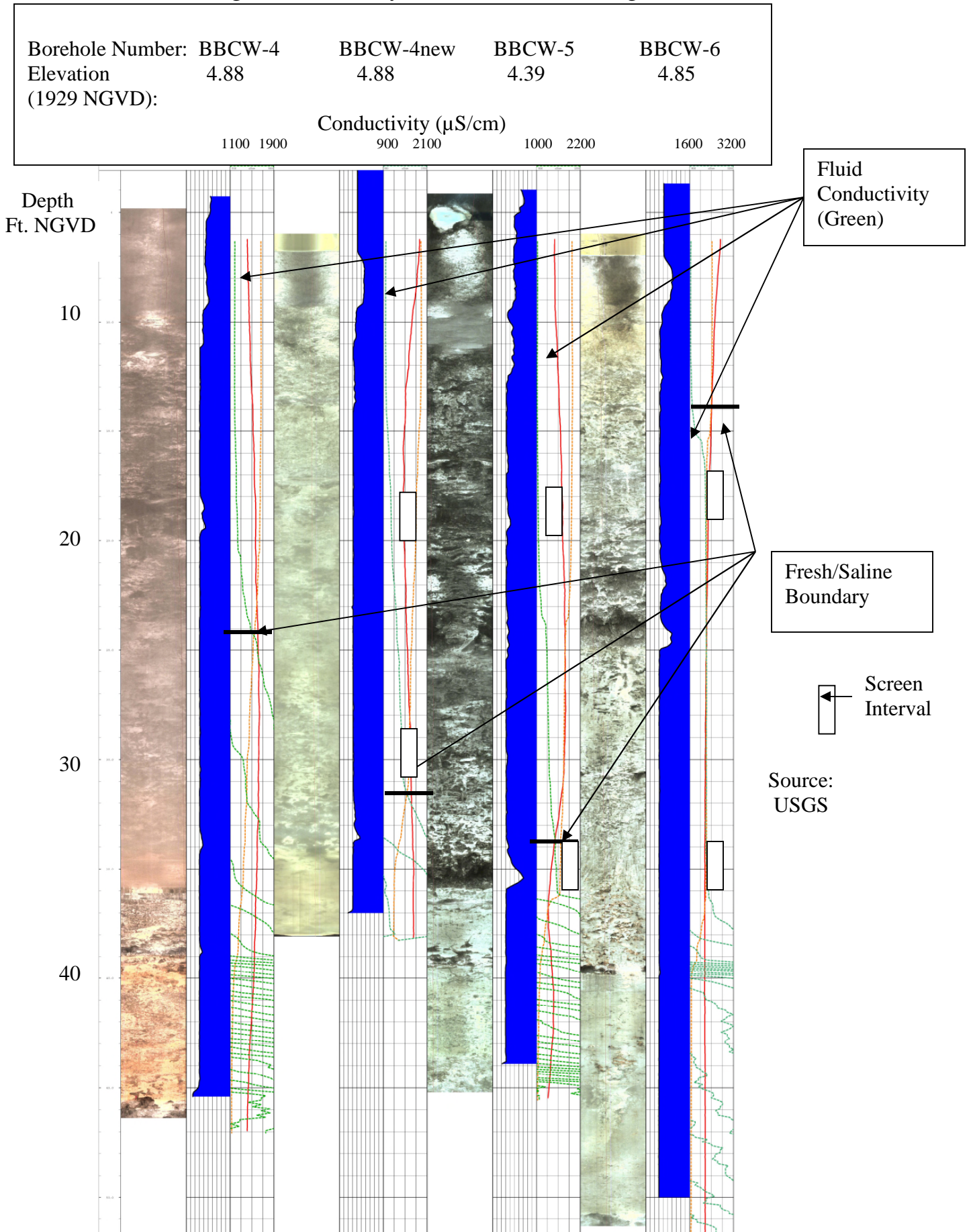
Figure 7 – Military Canal BBCW-4 through BBCW-6
