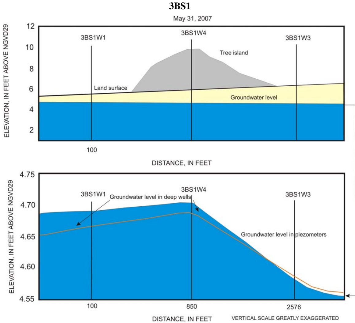
Figure 24 Cross section showing water levels in piezometers and deep wells at 3BS1 on May 31, 2007 (annual minimum).
